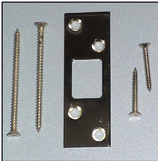
4-Screw Security Strike Plate (3-inch / 1 1/4 inch screws shown)
